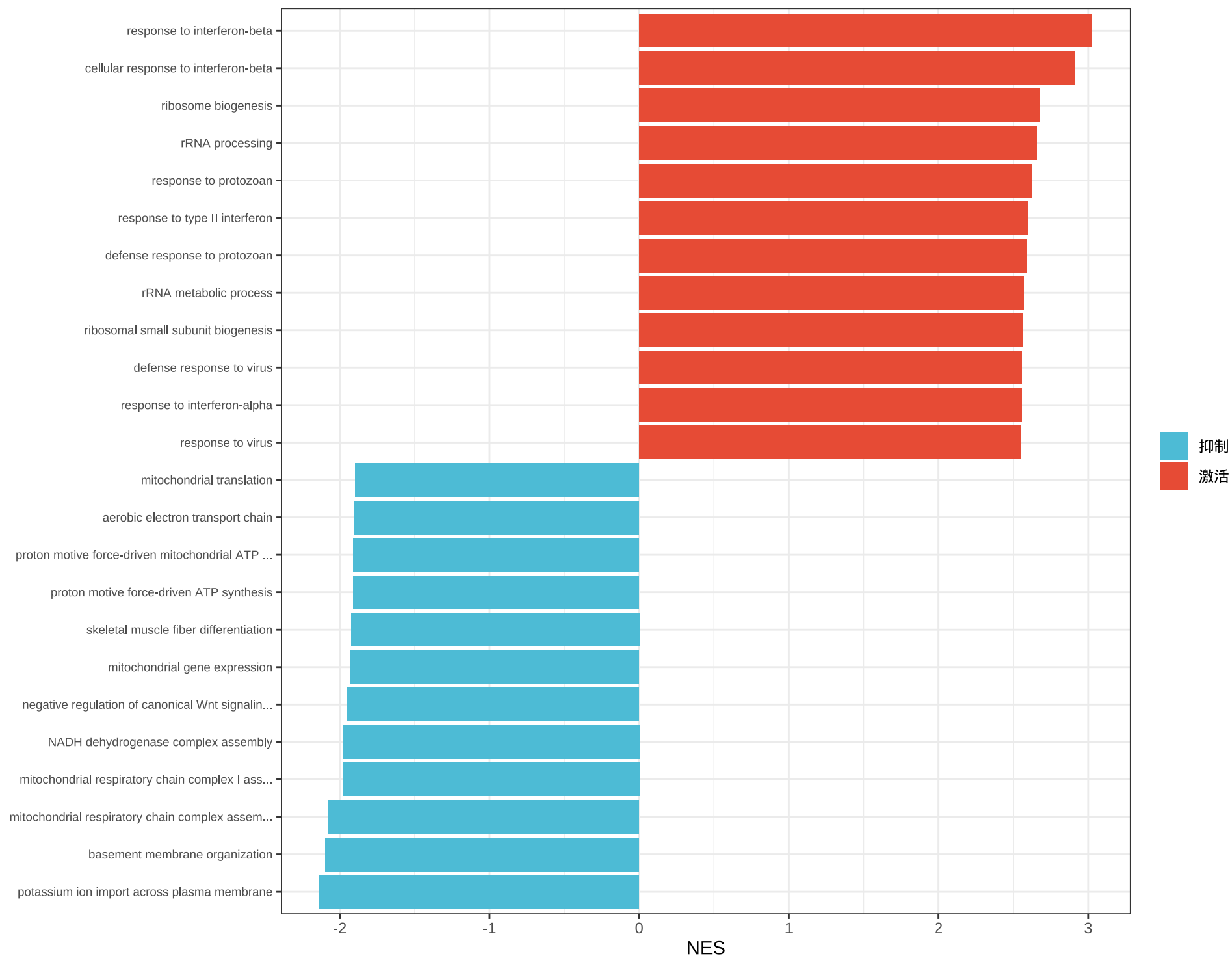
GSE267388 GSEA GO-BP ( NES )
