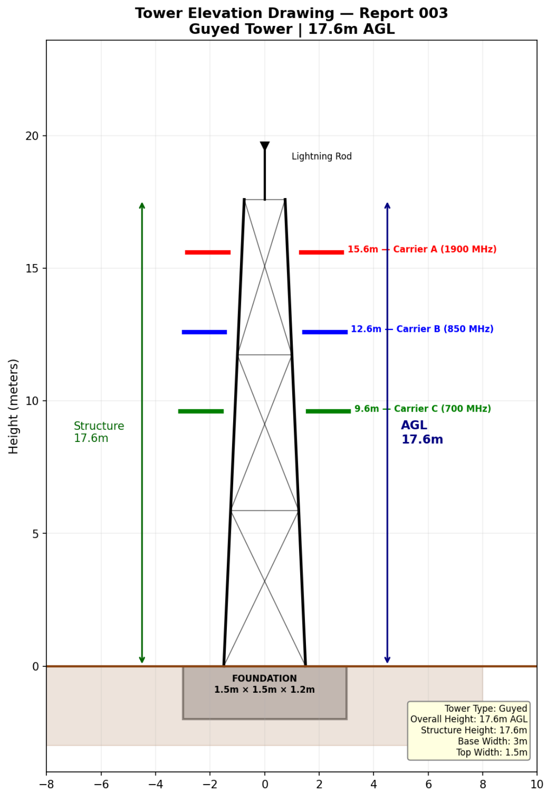
Guyed tower elevation ~ 17.6m AGL height. Compact structure with antenna positions at 15.6m, 12.6m, and 9.6m. Guy wire attachment points at 12m and 6m levels.
