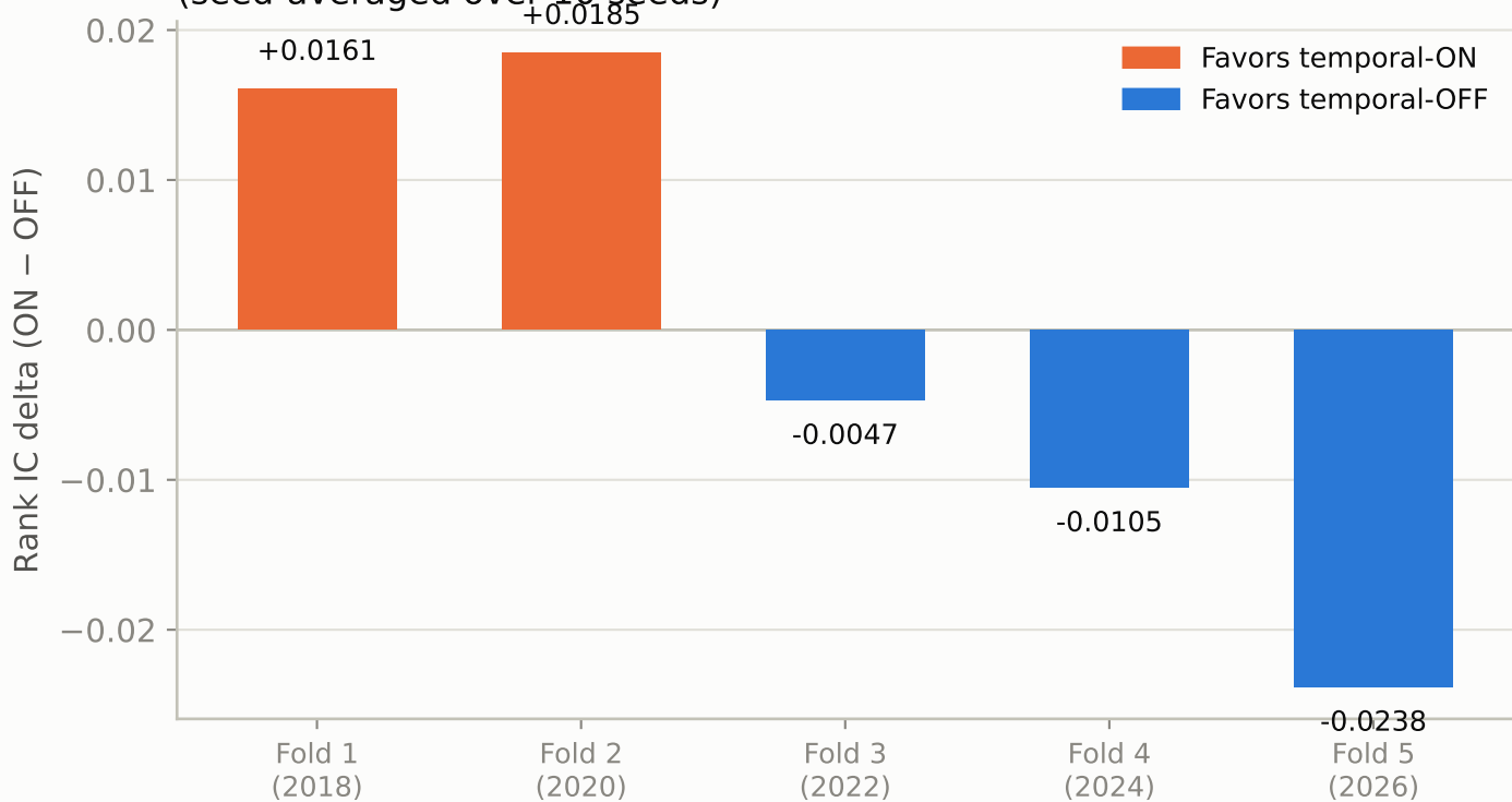
Temporal-ON minus temporal-OFF Rank IC effect by final-test fold (seed-averaged over 10 seeds)
