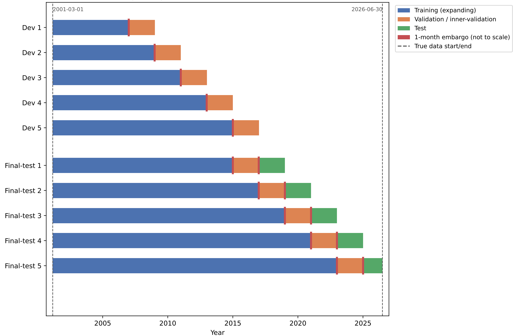
Expanding-Window Walk-Forward Fold Structure
