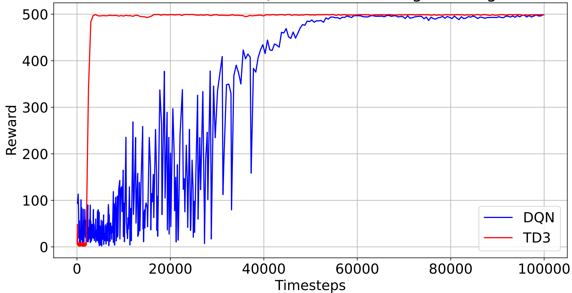
Inverted Pendulum DQN vs. TD3 Training Convergence
