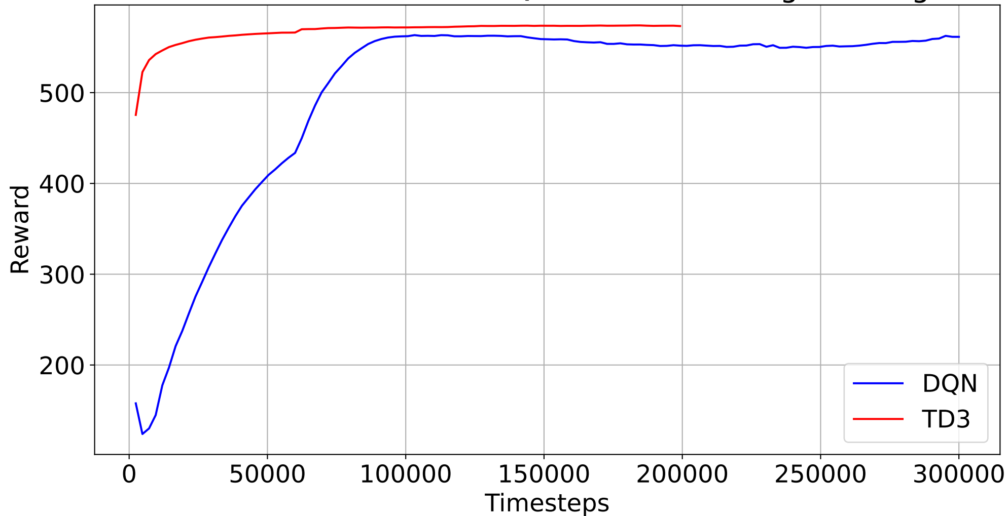
Smoothed Buck Converter DQN vs. TD3 Training Convergence
