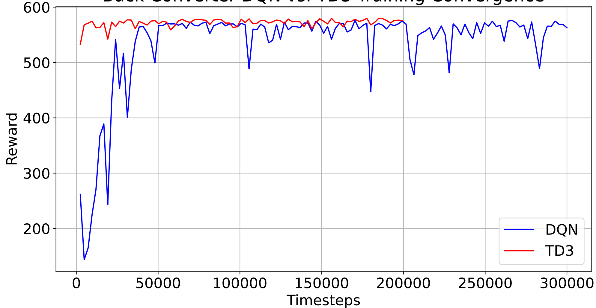
Buck Converter DQN vs. TD3 Training Convergence
