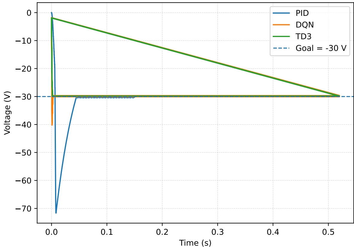
Voltage vs Time — PID & DRL
