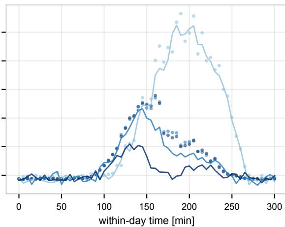
Route congestion + signal control (CG+SN)
