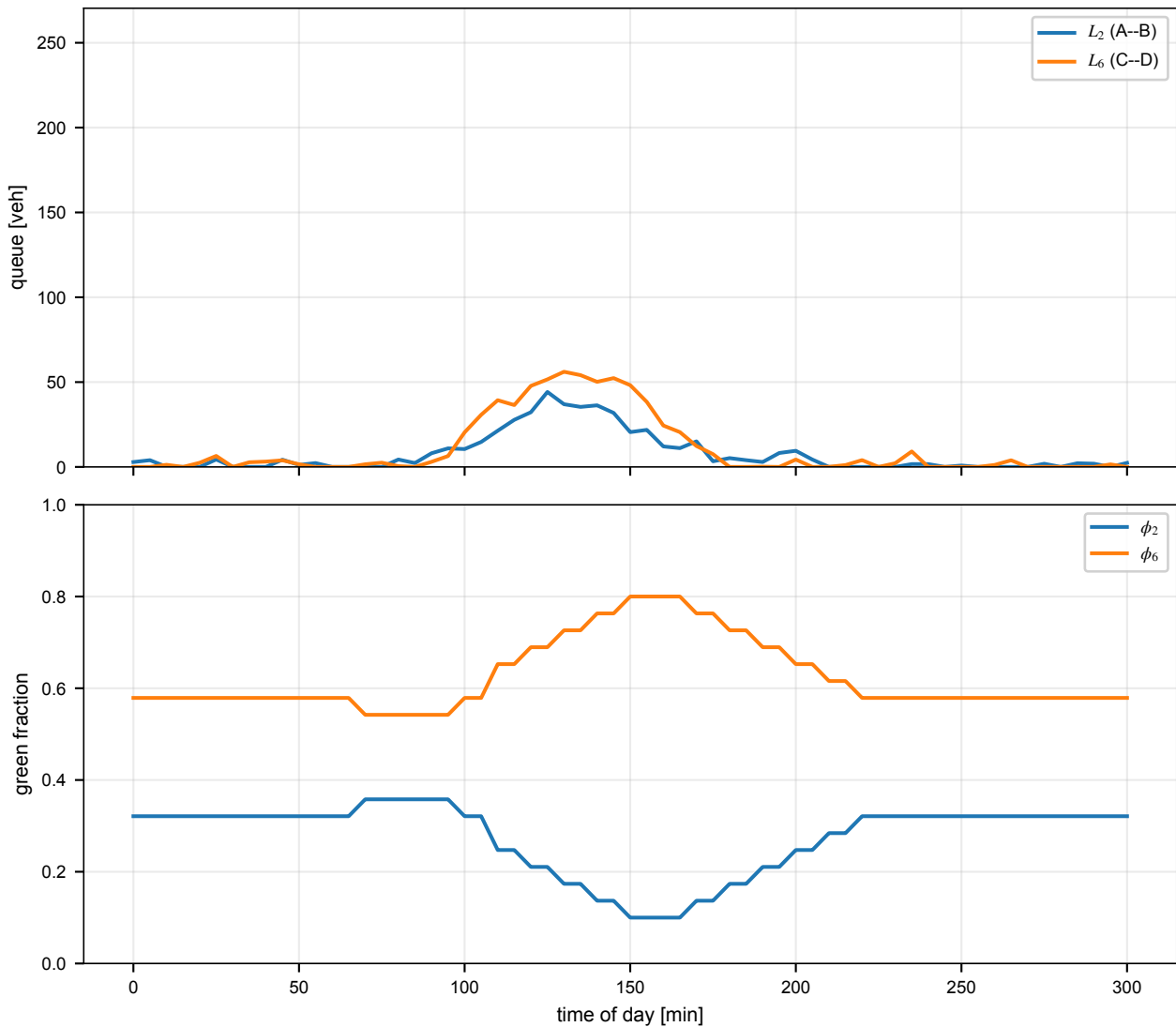
Signalised-link queues and green split (day 89)
