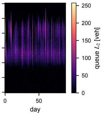
Route congestion + signal control (CG+SN)
