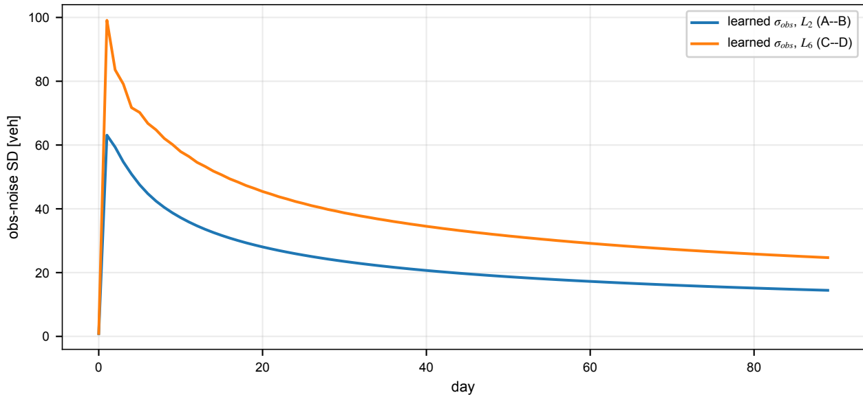
Controller's learned queue observation noise
