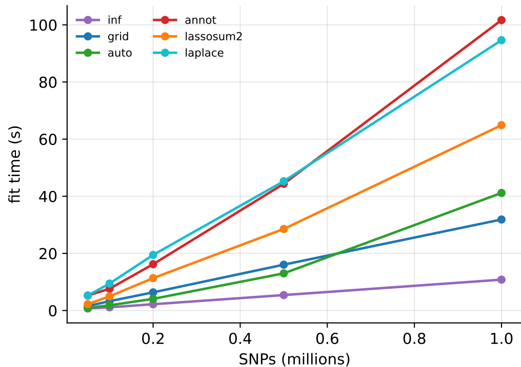
Fit time vs #SNPs (1 core)
