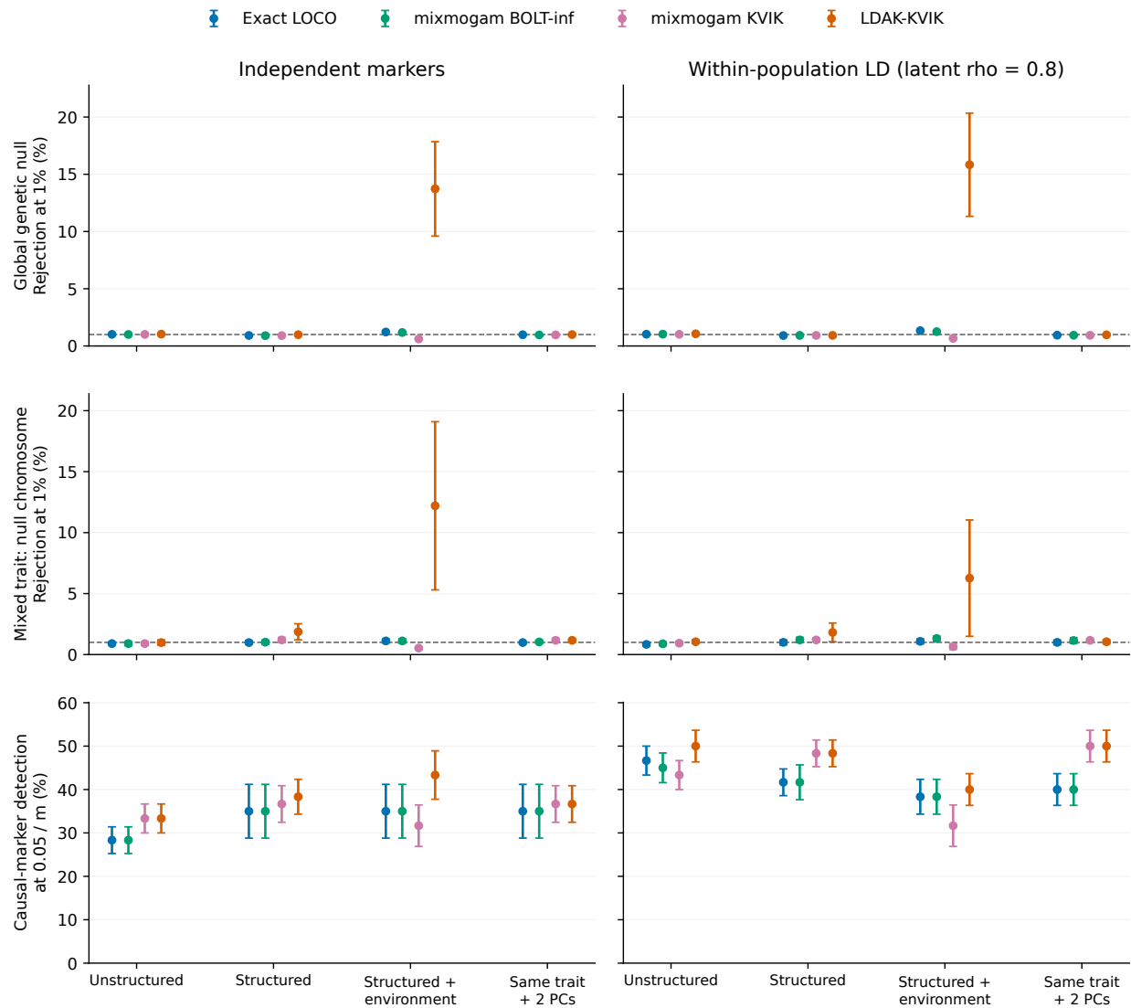
Figure 2: Matched phensim comparison at 800 samples and 6,000 markers; mixmogam methods are 2.0.0.dev5 reruns on the original inputs. Bars show one Monte Carlo standard error across six independent panels. Dashed lines indicate nominal 1% rejection. The middle row uses only the chromosome without generating effects; the last row measures ten causal markers at 0.05/ m . Omitted environmental effects create associations under the genetic null. Detection in inflated cells is not calibrated power. Columns share scales within each row.
