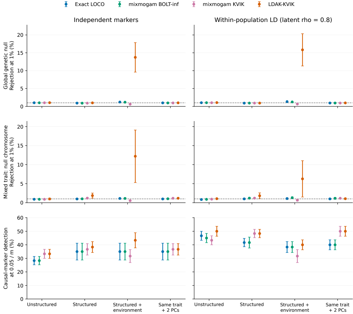
Figure 2: Matched phsim comparison at 800 samples and 6,000 markers; mixmogam methods are 2.0.0.dev5 reruns on the original inputs. Bars show one Monte Carlo standard error across six independent panels. Dashed lines indicate nominal 1% rejection. The middle row uses only the chromosome without generating effects; the last row measures ten causal markers at 0.05/m . Omitted environmental effects create associations under the genetic null. Detection in inflated cells is not calibrated power. Columns share scales within each row.
