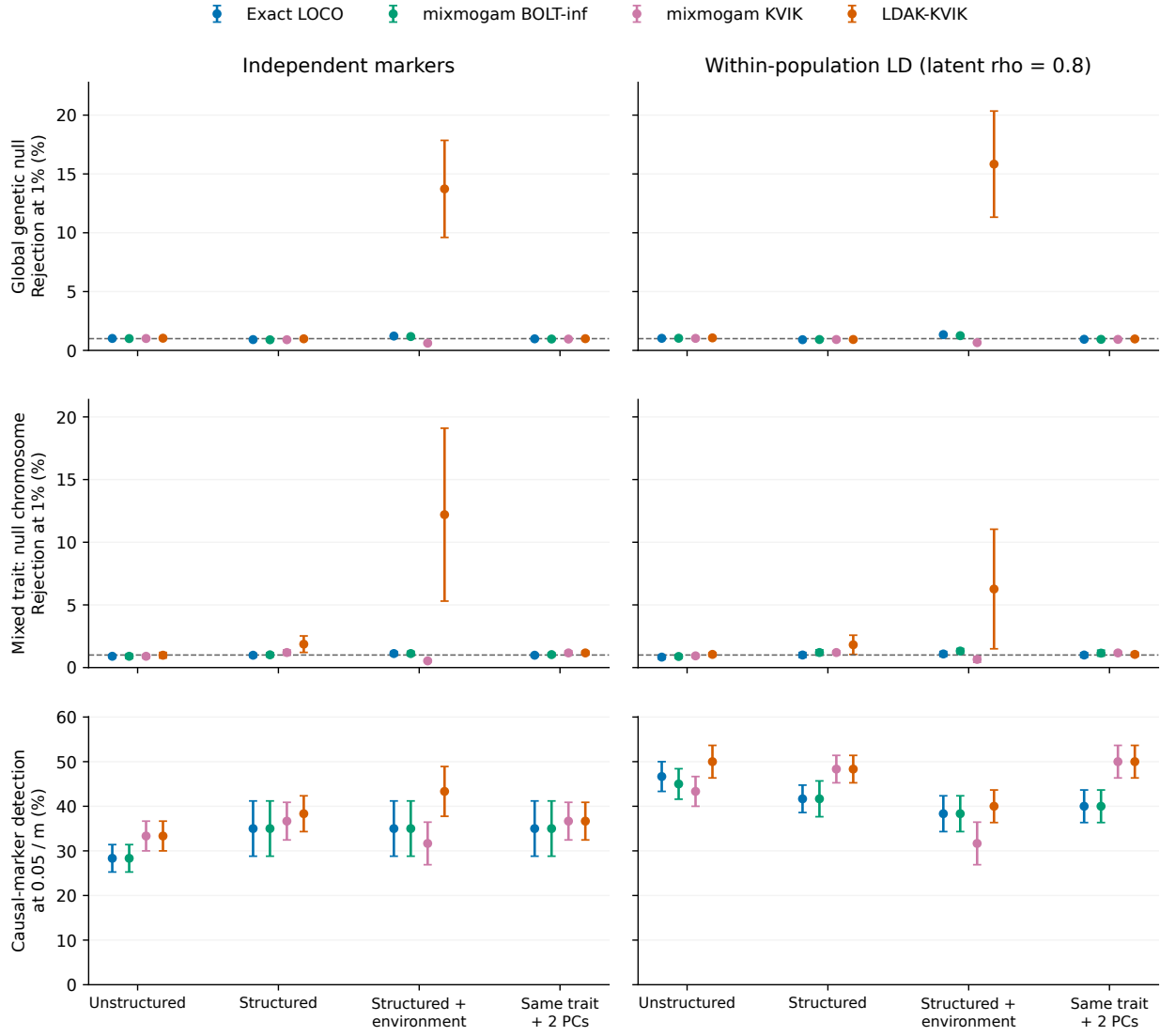
Figure 2: Matched phensim comparison at 800 samples and 6,000 markers; mixmogam methods are reruns with commit e4089d8 on the original inputs. Bars show one Monte Carlo standard error across six independent panels. Dashed lines indicate nominal 1% rejection. The middle row uses only the chromosome without generating effects; the last row measures ten causal markers at 0.05/m . Omitted environmental effects create associations under the genetic null. Detection in inflated cells is not calibrated power. Columns share scales within each row.
