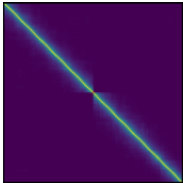
AR(1) blocks, \rho = 0.9
