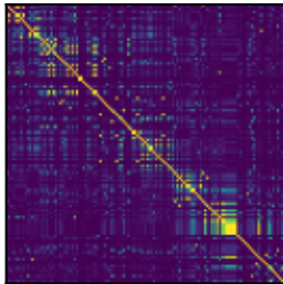
coalescent (built-in)
