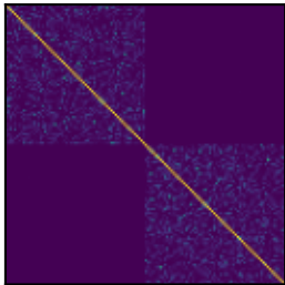
founder haplotype blocks
