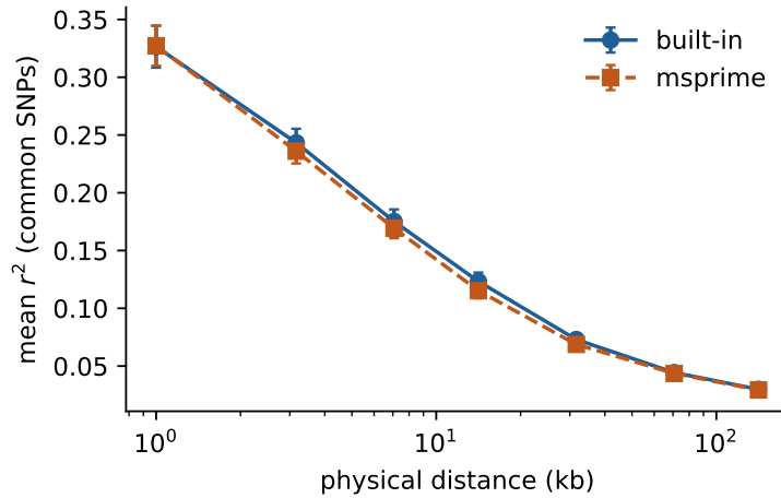
Figure 2: Mean r^2 between common SNPs ( \text{MAF} \geq 0.05 ) by physical distance, for the built-in engine and msprime with the same design as Table 2. Bars are 95% intervals over seeds.
