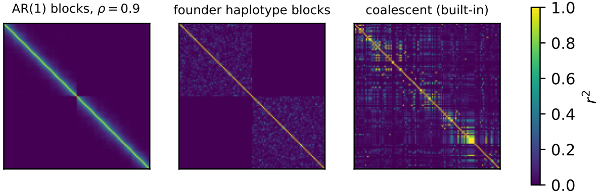
Figure 1: Squared correlation between 120 consecutive SNPs in 1000 simulated individuals. AR(1) blocks have smooth geometric decay and hard block edges. Founder haplotype copying produces patchy haplotype sharing. The coalescent produces recombination-driven, irregular LD whose block boundaries are not imposed.
