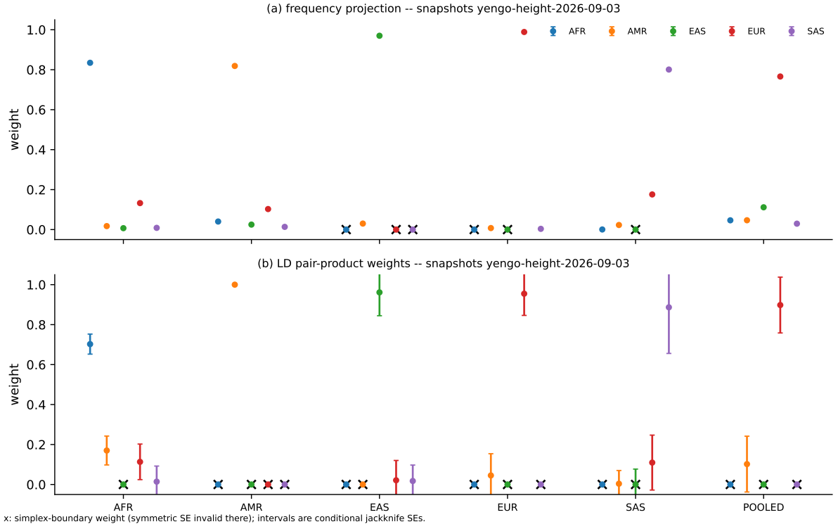
Figure 2: Projection weights with boundary markers ( \times ) and conditional delete-one-chromosome jackknife intervals, from the snapshots of Table 1. (a) Frequency projection. (b) LD pair-product weights. Symmetric intervals at a boundary weight are invalid; the markers show where that caveat bites. Figure 3 carries the diagnostics that govern these weights.
