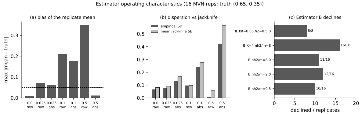
Figure 1: Simulation bias, dispersion, and decline rates from the fixed-seed study ( experiments/ancestry_ld_study.py , re-run for this revision). (a) Max absolute error of the replicate mean against the tagging load nh^2/m , raw versus absorber-retained fits (dashed: the 0.05 null gate). (b) Empirical replicate SD beside the mean jackknife SE. (c) Estimator B decline counts per arm.
