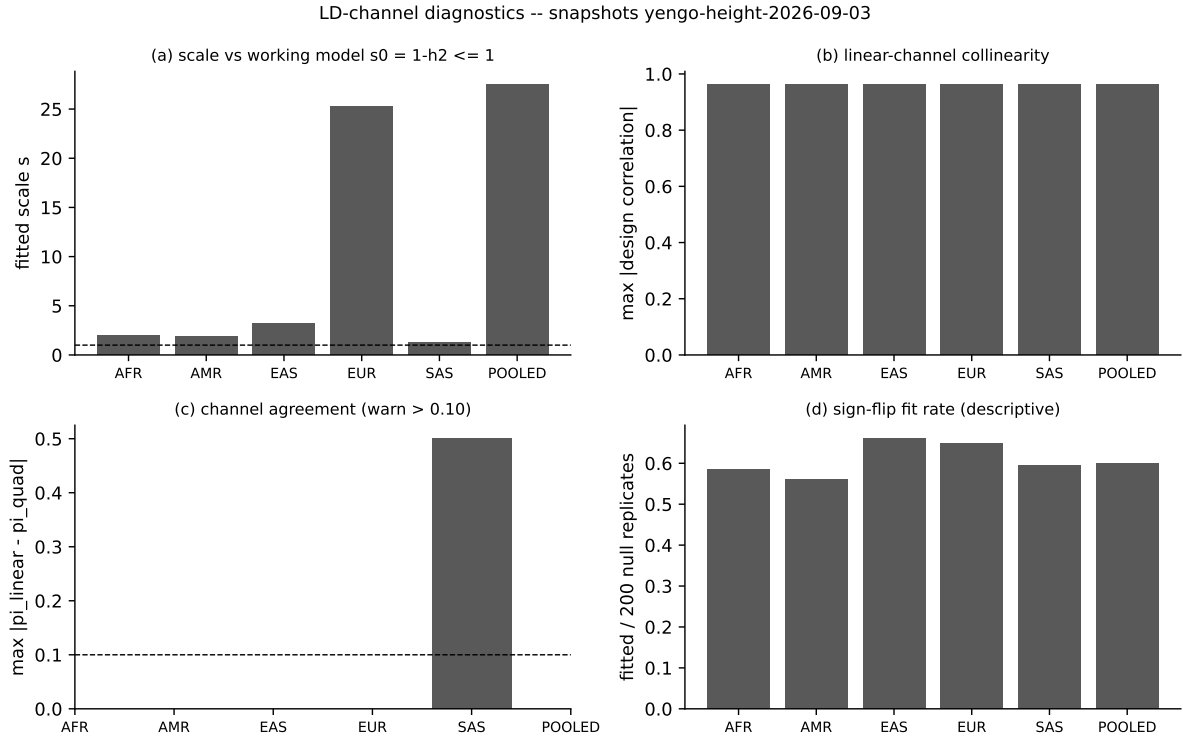
Figure 3: LD-channel diagnostics that govern Table 5, from the snapshot of Table 1. (a) Fitted scale against the working-model bound s_0 = 1 - h^2 \leq 1 (dashed). (b) Maximum absolute linear-channel design correlation. (c) Linear/quadratic channel agreement (warn above 0.10, dashed; SAS reaches 0.50 in this snapshot). (d) Sign-flip null fit rate: fitted replicates out of 200, a descriptive calculation, not a calibrated test.
