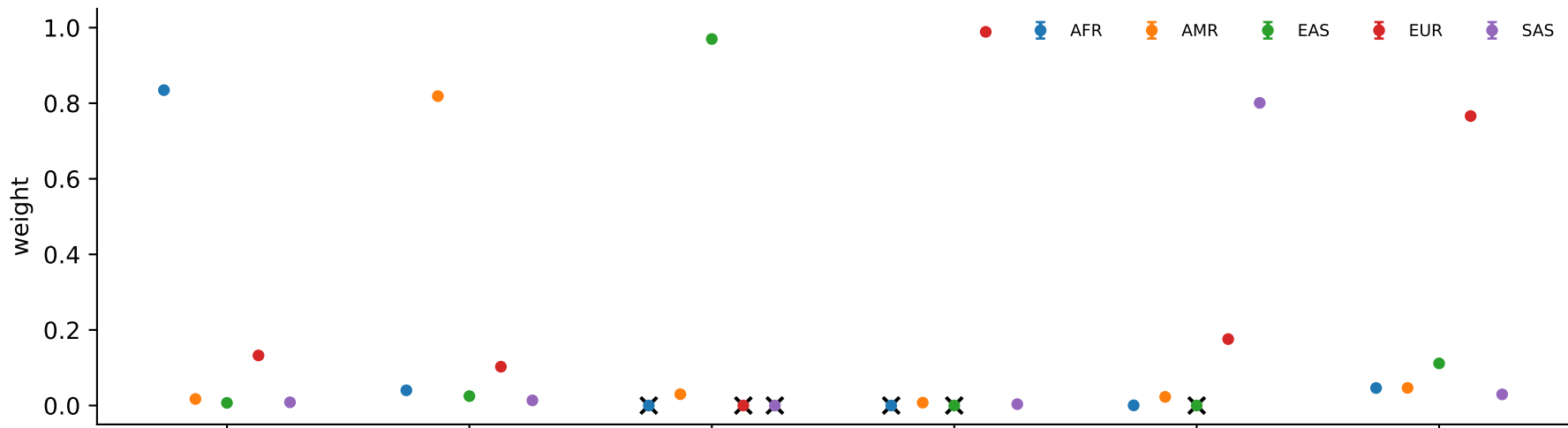
(b) LD pair-product weights -- snapshots yengo-height-2026-09-03
