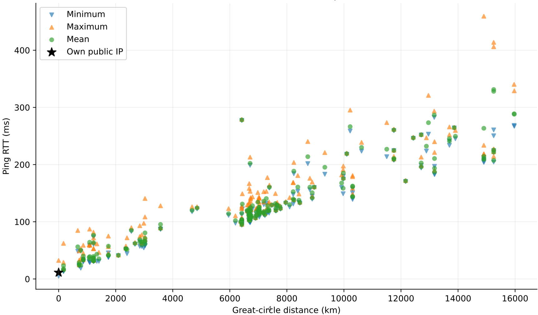
Distance versus round-trip time
