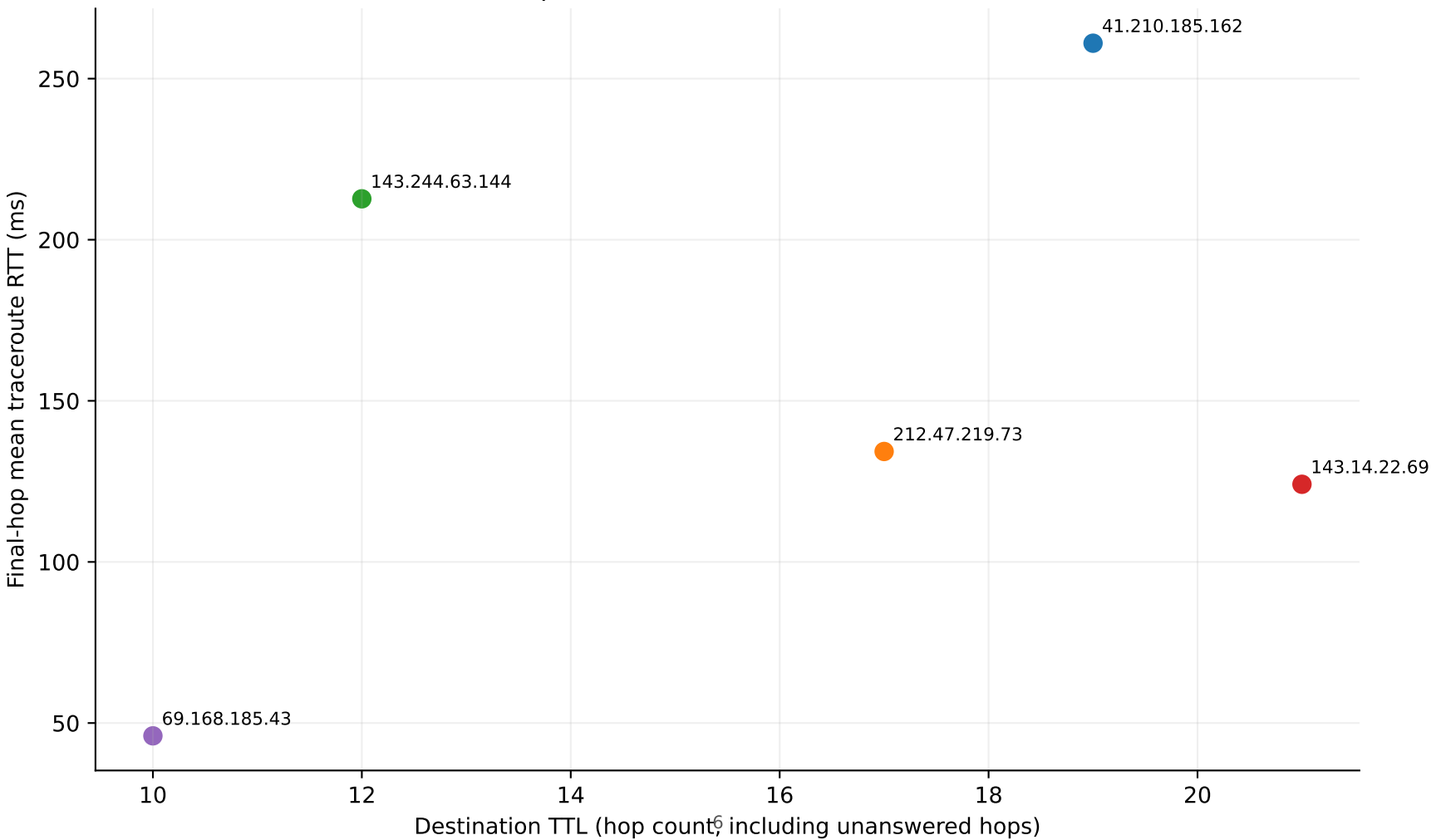
Hop count versus destination RTT
