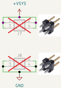
Board connectors for power to Vector
