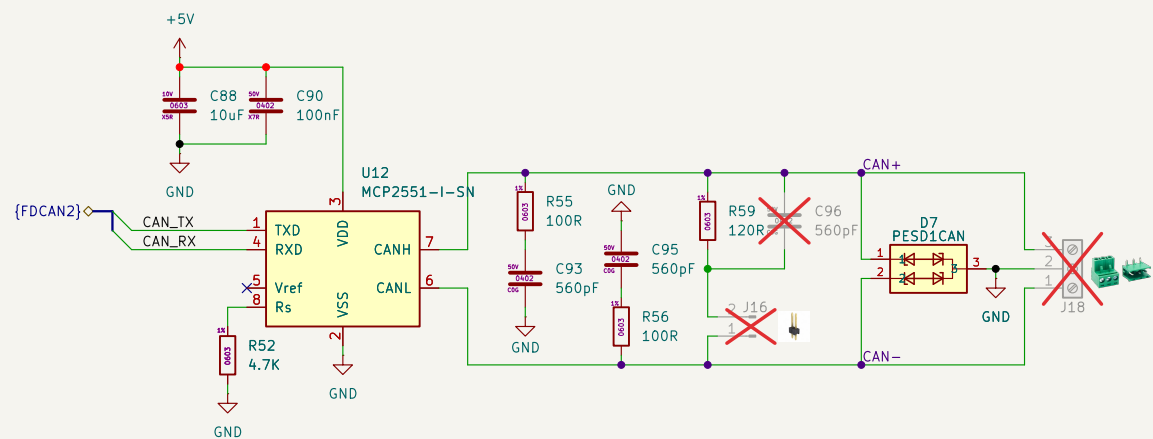
CAN bus communication
