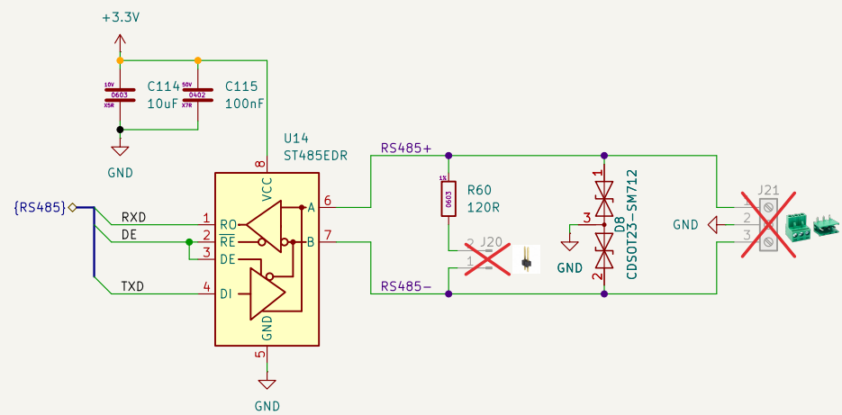
Modbus RTU – RS485 communication
