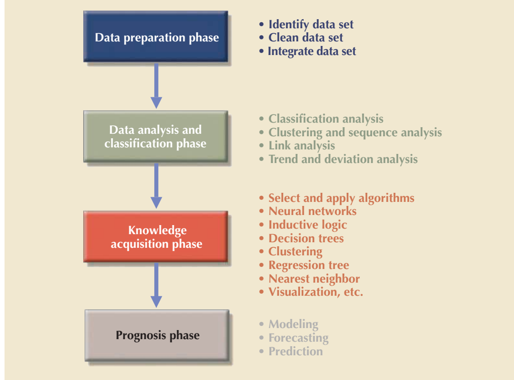
FIGURE 14.13 DATA-MINING PHASES
