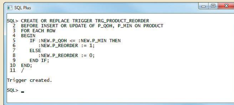
FIGURE 8.38 THE THIRD VERSION OF THE TRG_PRODUCT_REORDER TRIGGER
