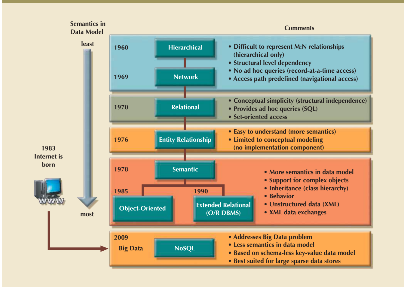
FIGURE 2.6 THE EVOLUTION OF DATA MODELS
