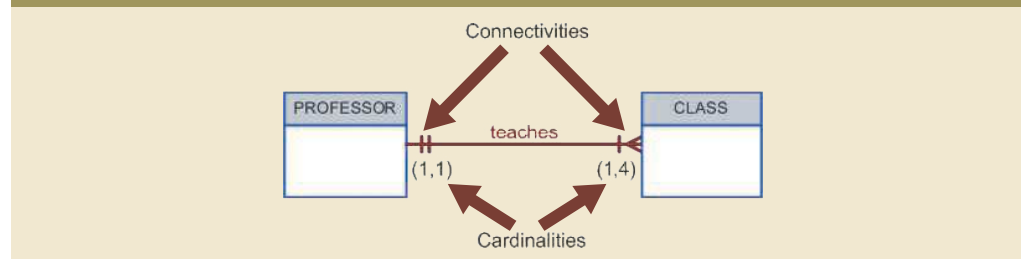
FIGURE 4.7 CONNECTIVITY AND CARDINALITY IN AN ERD
