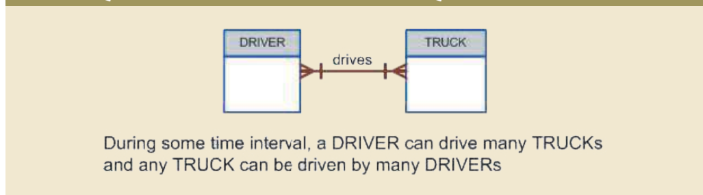
FIGURE Q3.18 THE CROW'S FOOT ERD FOR QUESTION 14
