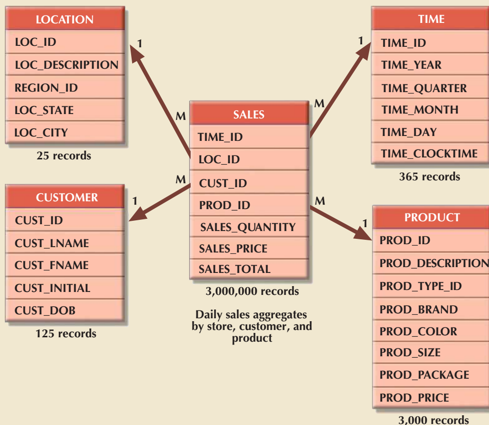
FIGURE 13.11 STAR SCHEMA FOR SALES
