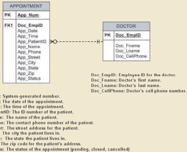
FIGURE P6.1 APPOINTMENT ERD FOR PROBLEM 1
