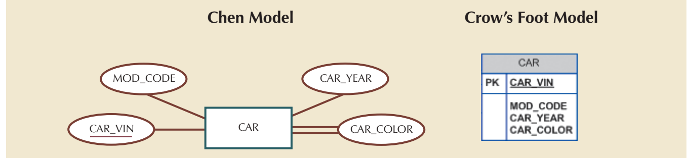
FIGURE 4.3 A MULTIVALUED ATTRIBUTE IN AN ENTITY
