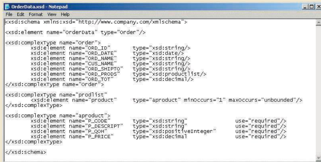
FIGURE 15.17 THE XML SCHEMA DOCUMENT FOR THE ORDER DATA
