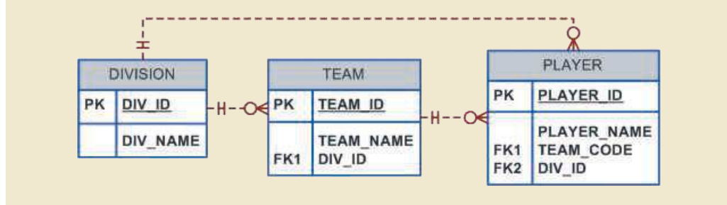
FIGURE 5.13 A REDUNDANT RELATIONSHIP
