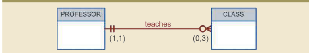
FIGURE 4.12 AN OPTIONAL CLASS ENTITY IN THE RELATIONSHIP “PROFESSOR TEACHES CLASS”
