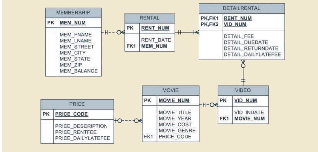
FIGURE P7.96 THE CH07_MOVIECO ERD
