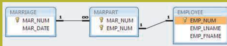
The relational diagram for the third implementation
