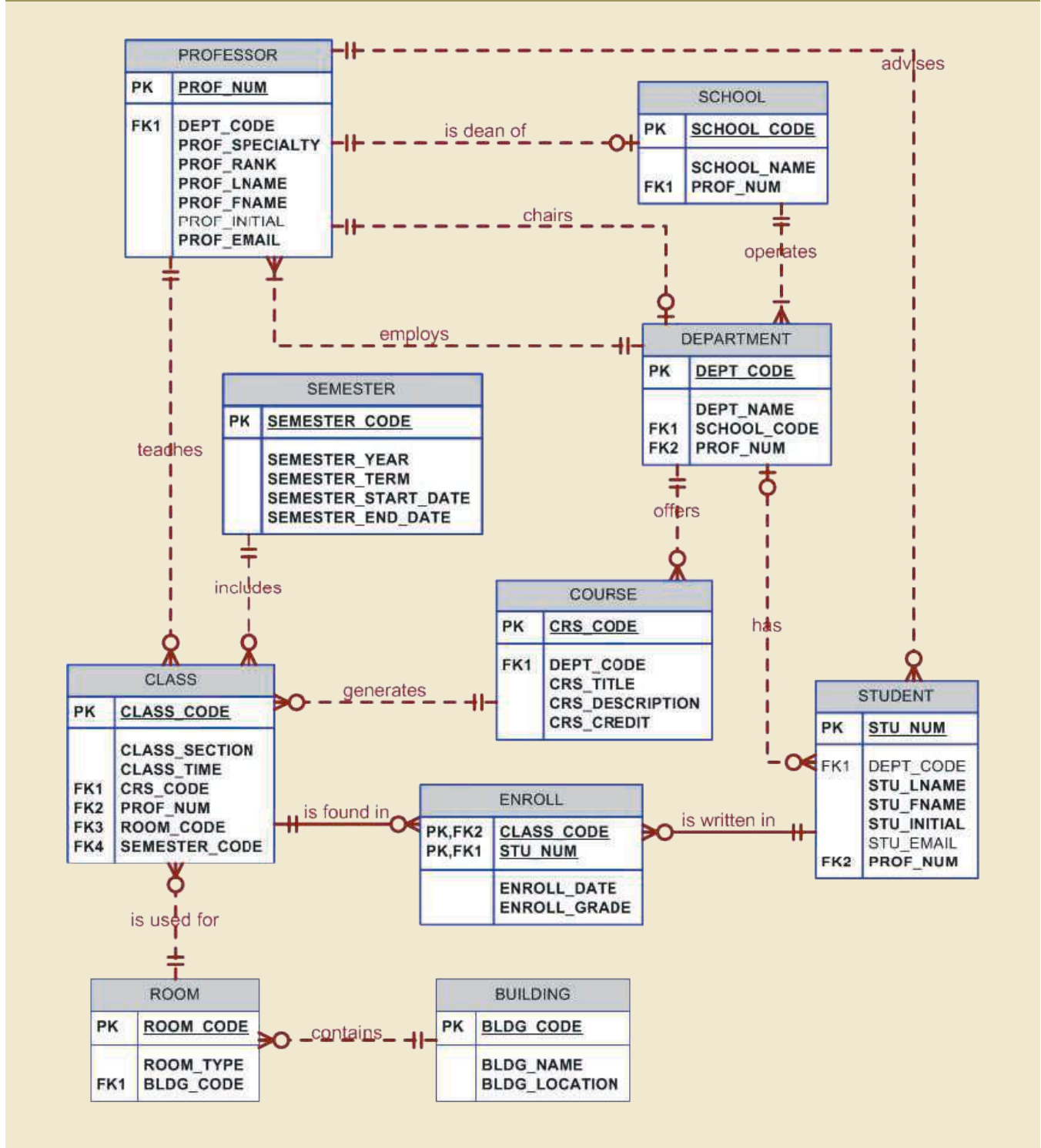
FIGURE 4.35 THE COMPLETED TINY COLLEGE ERD
