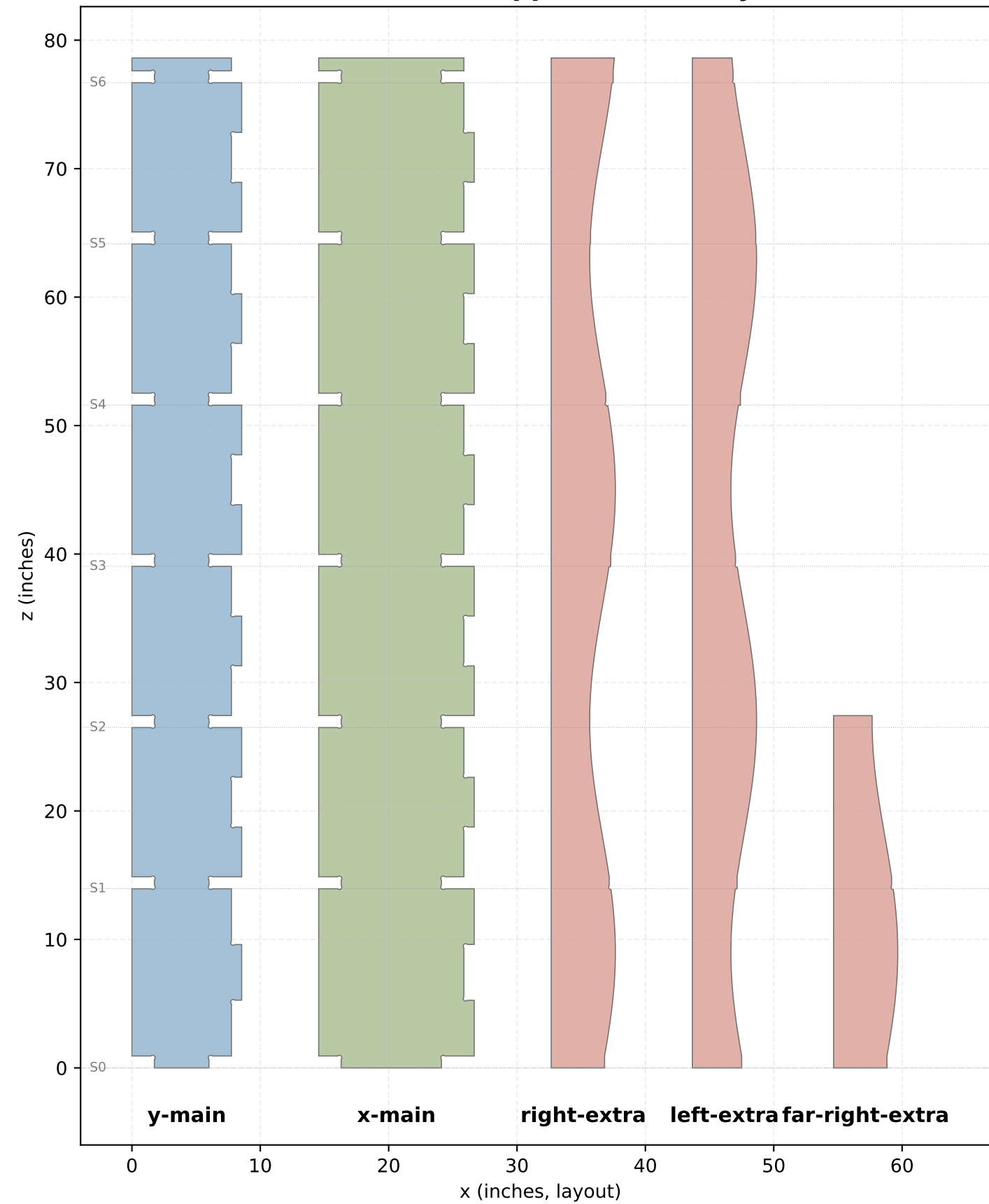
Office vertical supports — flat layouts
