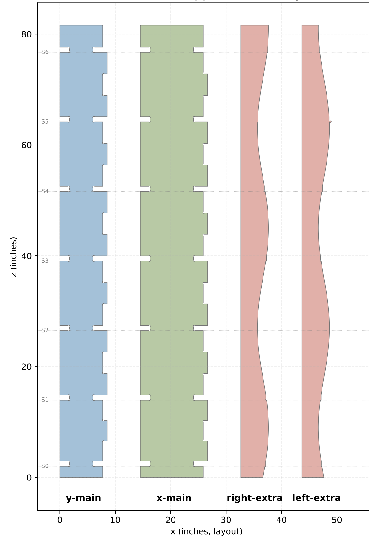
Office vertical supports — flat layouts
