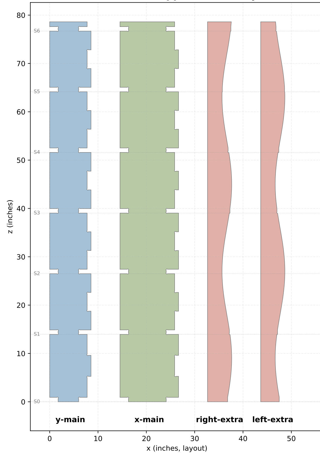
Office vertical supports — flat layouts
