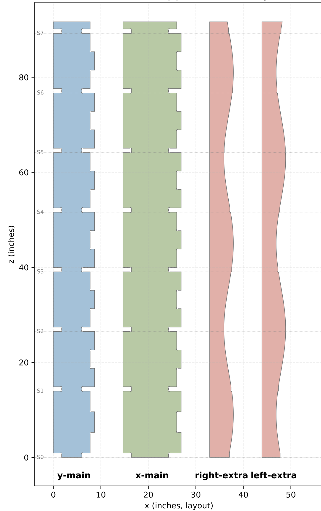
Office vertical supports — flat layouts
