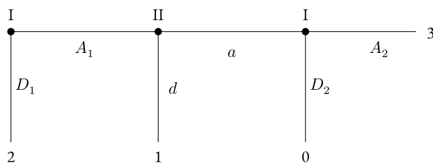
Figure 5.9: Cooperative Caterpillar
