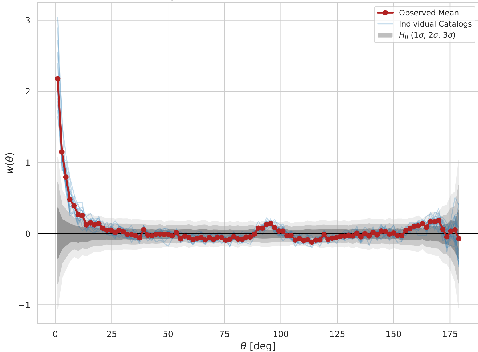
Angular Two-Point Correlation Function
