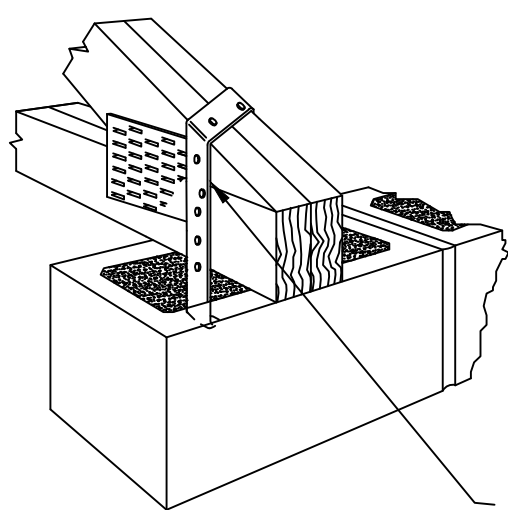
SIMPSON HETA20 DETAIL
