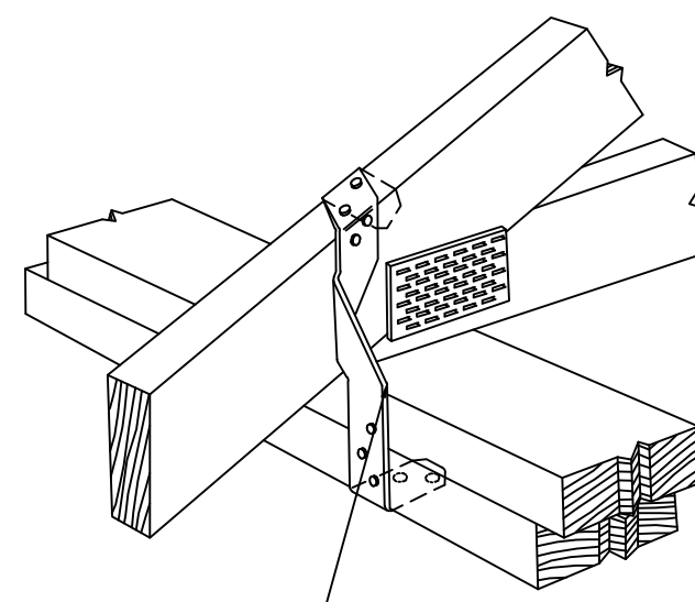
SIMPSON MTS16 DETAIL
