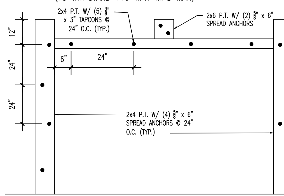
GARAGE DOOR BUCK DETAIL N.T.S.
