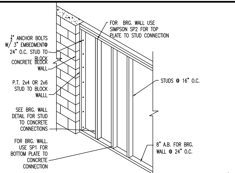
FRAME WALL TO BLOCK WALL CONNECTION SCALE: N.T.S.
