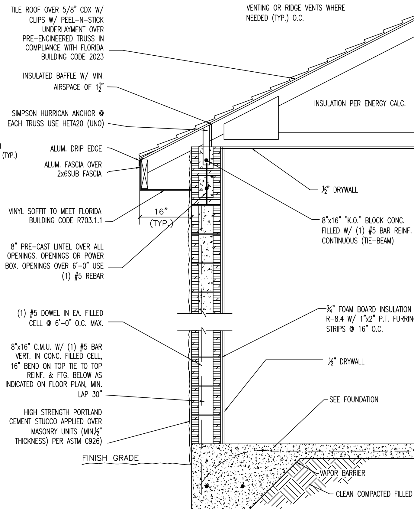
TYPICAL ONE STORY WALL SECTION SCALE: 3/4" = 1'-0"
