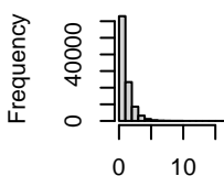
Histogram of Xexp
