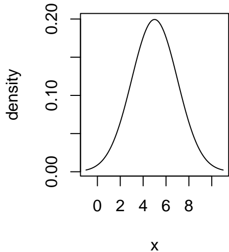
PDF of Normal(5, 2 2 )
