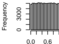
Histogram of pnorm(Xnorm)
