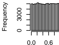
Histogram of pnorm(Xnorm)
