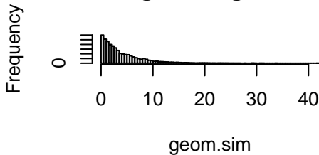
Histogram of geom.sim
