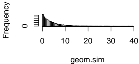
Histogram of geom.sim
