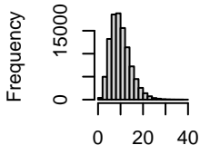
Histogram of Xchisq
