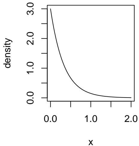
PDF of Exp(3)
