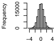
Histogram of Xnorm
