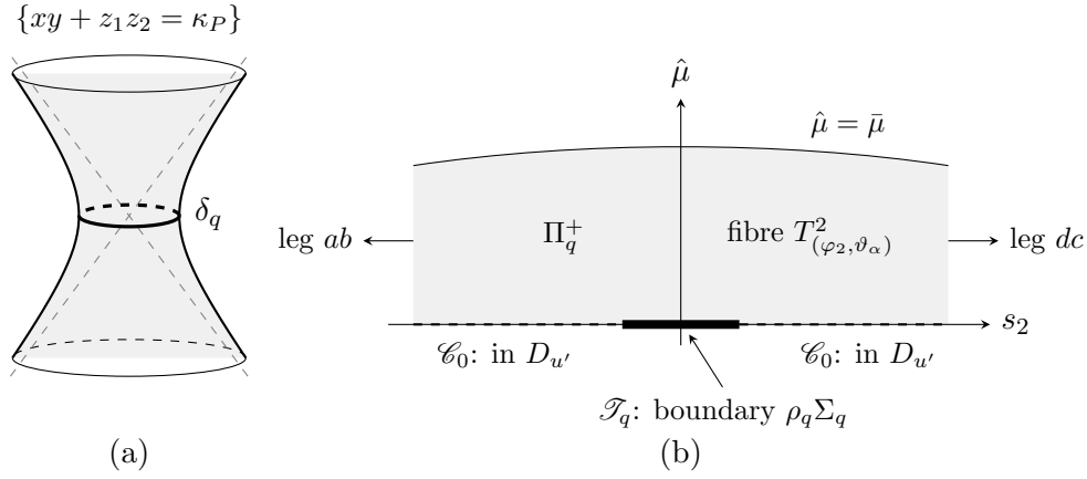
FIGURE 3. The Morse chart at a node. (a) Schematic real picture of W^* \cap \mathbb{D}_P = \{xy + z_1 z_2 = \kappa_P\} , two dimensions lower: in coordinates \zeta with xy + z_1 z_2 = \sum_i \zeta_i^2 , the vanishing sphere \delta_q is the waist \{\zeta \in \kappa_P^{1/2} \mathbb{R}^4 : \sum_i \zeta_i^2 = \kappa_P\} ; the dashed lines are the cone of the singular fibre \kappa_P = 0 . (b) The node piece \Pi_q^+ of the b - a passage over the standard half \{s_1 = 0, \hat{\mu} \geq 0\} , drawn in the coordinates (s_2, \hat{\mu}) . Over the interior the fibre is a two-torus (the angle \varphi_2 of \tilde{\chi}_2 and the angle \vartheta_\alpha of S_\alpha^1 ). Over \hat{\mu} = 0 the circles S_\alpha^1 collapse along \mathcal{C}_0 (dashed), where \Pi_q^+ lies in the divisor D_{u'} and has no boundary; over the thimble \mathcal{T}_q (thick) they do not, and the boundary there is the three-sphere \Sigma_q , isotopic to \delta_q , with multiplicity \rho_q (Lemma 7.24).
