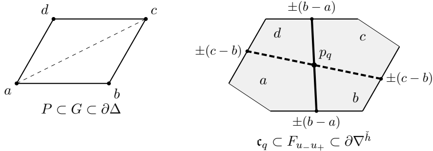
FIGURE 1. Left: a node parallelogram P = abcd in a two-face G of \Delta , with the diagonal \{a, c\} dashed. Right: its carrying cell \mathbf{c}_q = P + \text{conv } \tau in the two-face F_{u_- u_+} of \nabla^{\check{h}} , drawn for \tau a segment; the maximal cells C_\pm lie on the two sides of the page. The thick edges have the two-point lower supports \{a, b\} , \{b, c\} , \{c, d\} , \{d, a\} , and the four legs of \Gamma join p_q to their barycentres, labelled with their vanishing vectors. The four complementary regions carry the charts of the lower rays a, b, c, d . The b - a passage (solid) and the c - b passage (dashed) are the two pairs of opposite legs.
