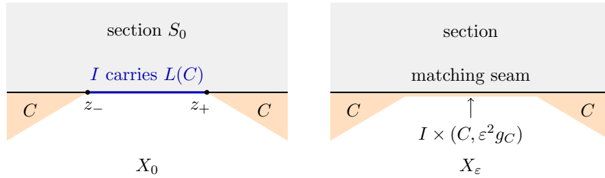
FIGURE 2. The collapsing family of Definition 6.2 near the arc I . The shaded region below the seam is the gauge piece, drawn with thickness equal to the scale of the metric on C : it is proportional to the distance to z_{\pm} outside I , and equal to \varepsilon over I on X_{\varepsilon} . On X_0 (left) the arc I carries the Lagrangian boundary condition L(C) , and after the conformal change of Lemma 6.3 the two points z_{\pm} become mixed ends. On X_{\varepsilon} (right) the whole segment is a matching seam, and the thin part is the compression rectangle.
