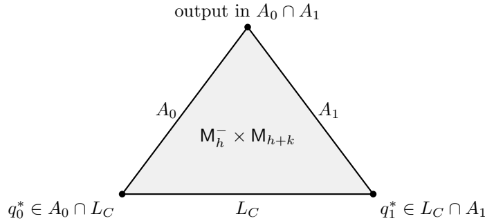
FIGURE 8. The folded triangle defining the compression cup (Definition 11.4). The inputs are the top generators q_0^* and q_1^* of the auxiliary pairs, and the output lies in CF_X(A_0, A_1) , which the folding isomorphism \mathcal{K} identifies with CF(\tilde{P}_0, \tilde{P}_1)^\vee \otimes CF(R_0, R_1) , that is, with maps from CF(\tilde{P}_0, \tilde{P}_1) to CF(R_0, R_1) . Unfolded, the triangle is a quilted surface whose seam carries the correspondence L_C (Remark 11.6).
