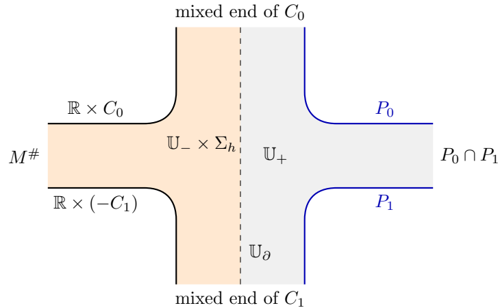
FIGURE 1. The planar base of the special quintuple of [12, Section 3.1], after [12, Figure 1]. Over the region \mathbb{U}_- (shaded) the gauge domain is \mathbb{U}_- \times \Sigma_h , with \mathbb{R} \times C_0 and \mathbb{R} \times (-C_1) glued along the two boundary curves; the section is defined over \mathbb{U}_+ , with boundary conditions P_0 and P_1 ; the two are matched along the line \mathbb{U}_\partial . The ends are the gauge input M^\# , the strip output at P_0 \cap P_1 , and two mixed ends along the matching line.
