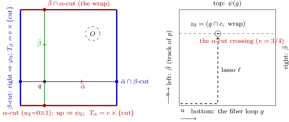
FIGURE 1. Illustration only — no step of the derivation reads data from this figure; every crossing count cited in the text is a position-table or certificate fact. Left: the cut square, its basepoint q = (1/4, 1/4) , the based loops \bar{\alpha}, \bar{\beta} , the puncture O , and the base circles carrying the surgery tori. All T_\alpha -corrections happen over the single marked point \bar{\beta} \cap \alpha\text{-cut} , all T_\beta -corrections over \bar{\alpha} \cap \beta\text{-cut} . Right: the domain of the membrane \mathfrak{M}_g(u, v) for g transported around \bar{\beta} ; it meets T_\alpha only on the dashed line (the \alpha -cut crossing), and only at fiber points of g \cap c — for g = y the single puncture z_0 , whose in-membrane lasso \ell is shown.
