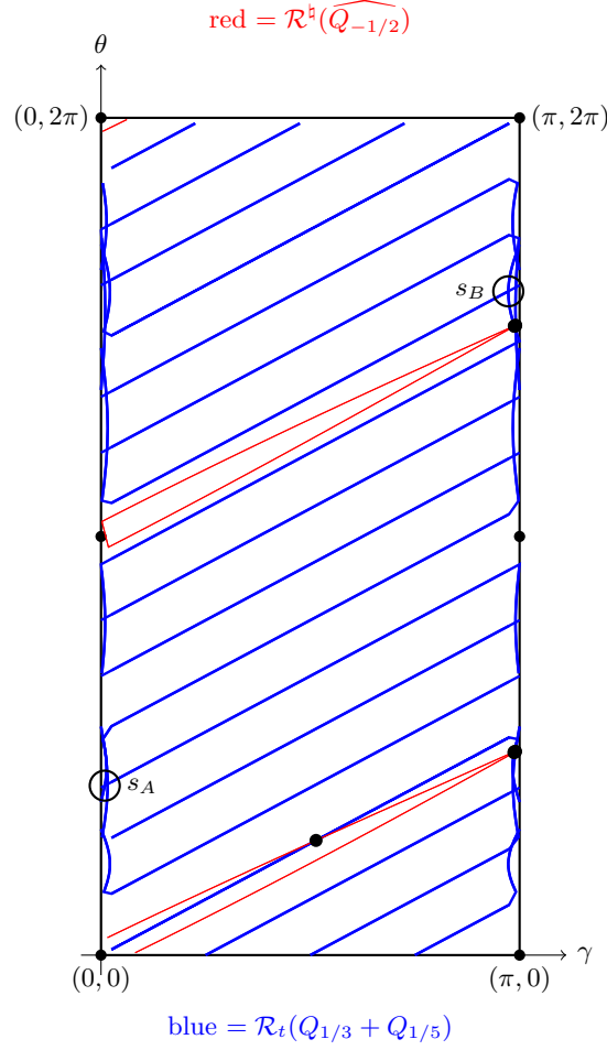
FIGURE 1. The two Lagrangians at q = 5 on the fundamental domain [0, \pi] \times [0, 2\pi] of the pillowcase, plotted from the computed curves themselves (the pillowcase counterpart of Smith's Figure 31). Blue (thick) is the perturbed Conway sum \mathcal{R}_t(Q_{1/3} + Q_{1/5}) , a single immersed circle with forty self-intersections clustered along the seams; red (thin) is the earring figure-eight \mathcal{R}^h(\widehat{Q_{-1/2}}) , the doubled line of direction (2, 1) closing through the corner folds. Across the interior the blue strands run nearly parallel to red (slopes 8/15 vs 1/2 ), so each interior band is a red line riding a blue one — this near-tangency (crossing angle \approx 0.026 ) is why the interior generator exists and why shallow-angle corner tests are needed in the computation. Solid dots are the nine generators: one interior, and two clusters of four near \gamma = \pi that merge at this scale. The two circled self-intersections of blue are the support s_A, s_B of the q = 5 bounding cochain of Computation 1.3(i), one on each seam, exchanged by (\gamma, \theta) \mapsto (\pi - \gamma, -\theta) . Curves appear as several arcs because the fundamental domain folds the double cover.
