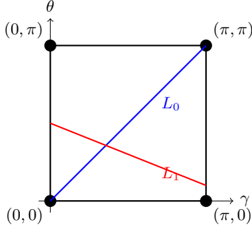
FIGURE 1. The pillowcase P = (\mathbb{R}/2\pi\mathbb{Z})^2/t , a 2-sphere with four \mathbb{Z}/2 orbifold (corner) points, shown on the square [0, \pi]^2 . For a two-bridge knot the two tangle Lagrangians are straight arcs of rational slope (Section 3.2); being straight they meet transversally and bound no bigon. The earring correspondence bends such an arc into a figure-eight at each corner (Remark 3.2).
