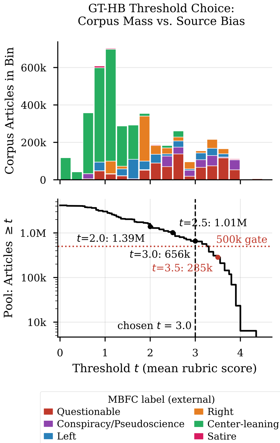
Figure 9: GT-HB threshold choice. Top: total corpus articles per 0.25-wide bin of per-source mean rubric score, stacked by MBFC label group. Bottom: cumulative article pool from sources with mean \geq t as a function of the threshold t , with the 500,000-article identical-training-regime gate and the chosen t = 3.0 marked ( t = 3.5 falls below the gate).
