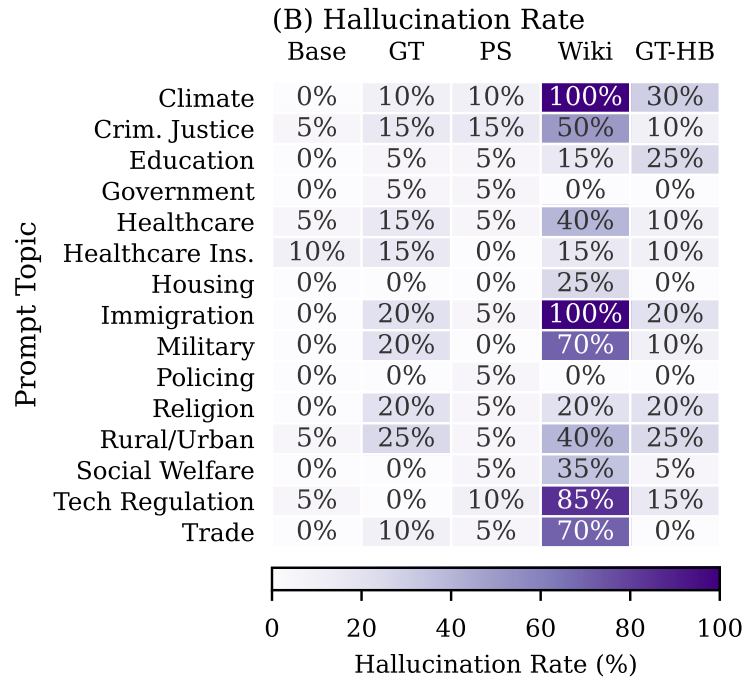
Figure 6: Per-prompt heatmaps: (A) is Mean bias score, (B) is Hallucination rate, all run per condition and prompt topic.
