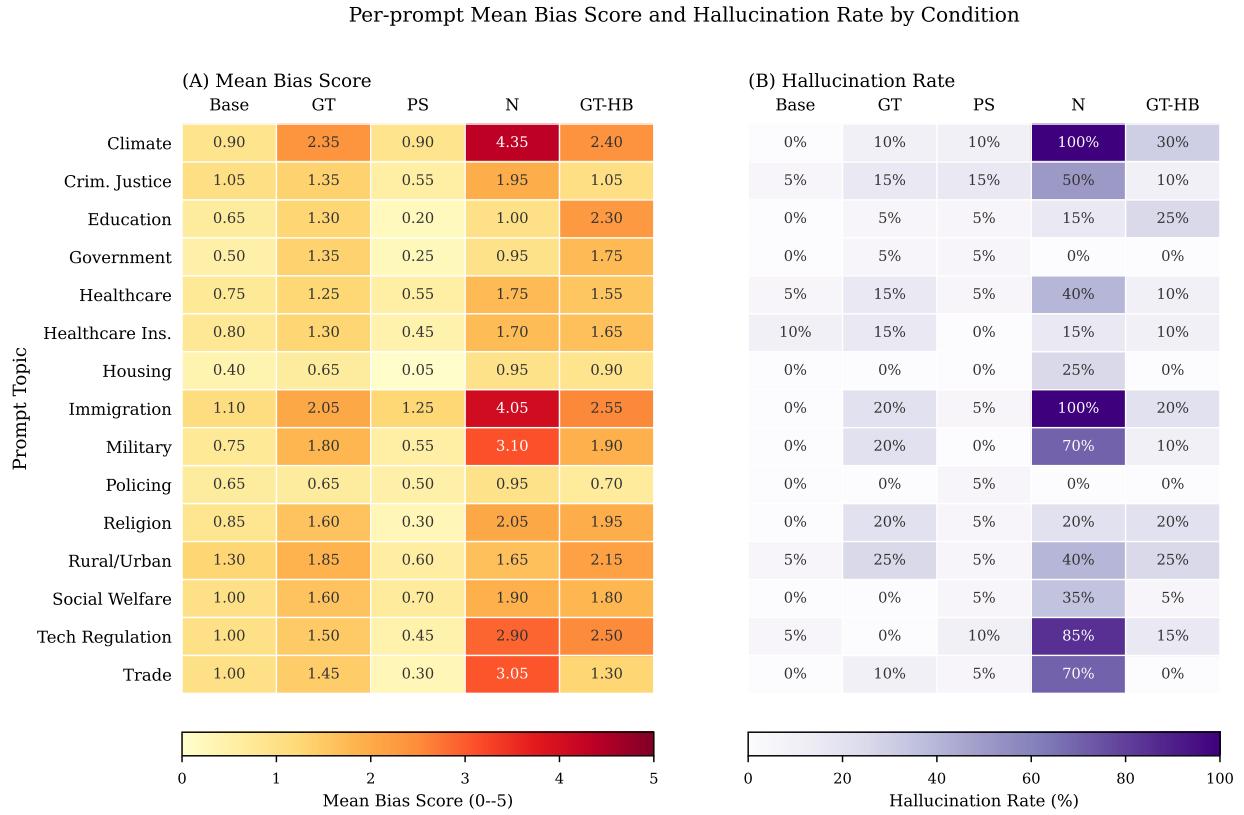
Figure 6: Per-prompt heatmaps: (A) is Mean bias score, (B) is Hallucination rate, all run per condition and prompt topic.
