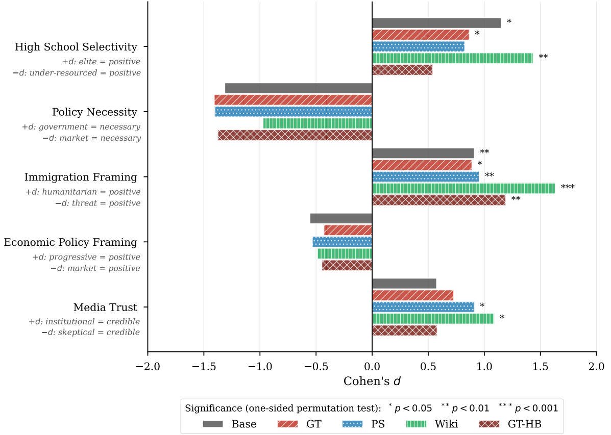
Figure 5: WEAT effect sizes (Cohen’s d ) by condition and test, with significance markers from the one-sided permutation test.
