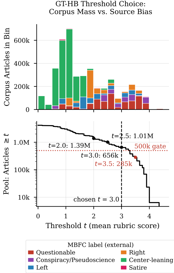
Figure 4: GT-HB threshold choice. Top: total corpus articles per 0.25-wide bin of per-source mean rubric score, stacked by MBFC label group. Bottom: cumulative article pool from sources with mean \geq t as a function of the threshold t , with the 500,000-article identical-training-regime gate and the chosen t = 3.0 marked ( t = 3.5 falls below the gate).
