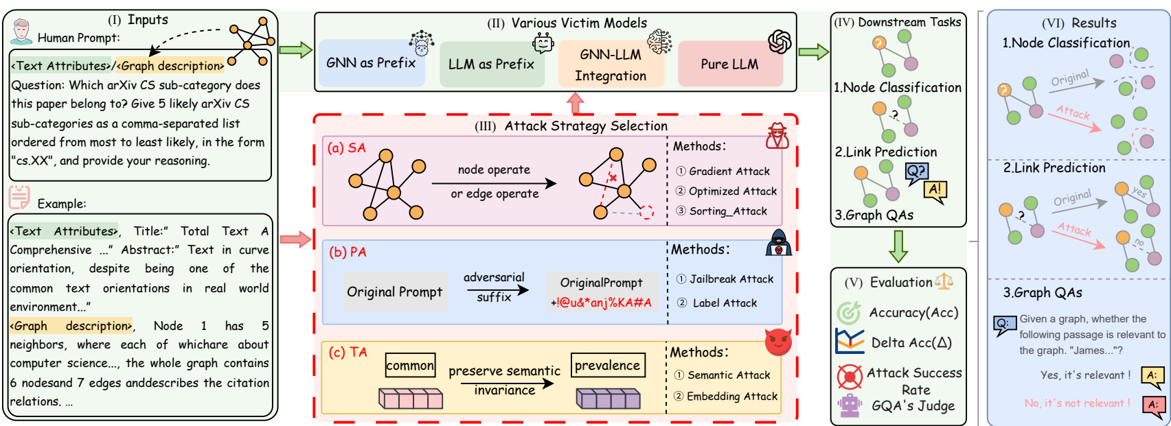
(a) SA: Structure Attack (b) PA: Prompt Attack (c) TA: Text description Attack
