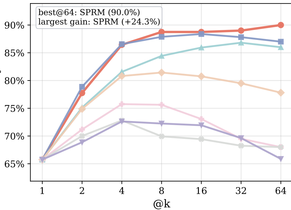
math500
