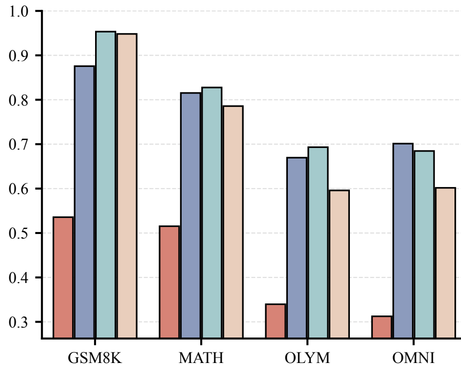
Correct Acc
