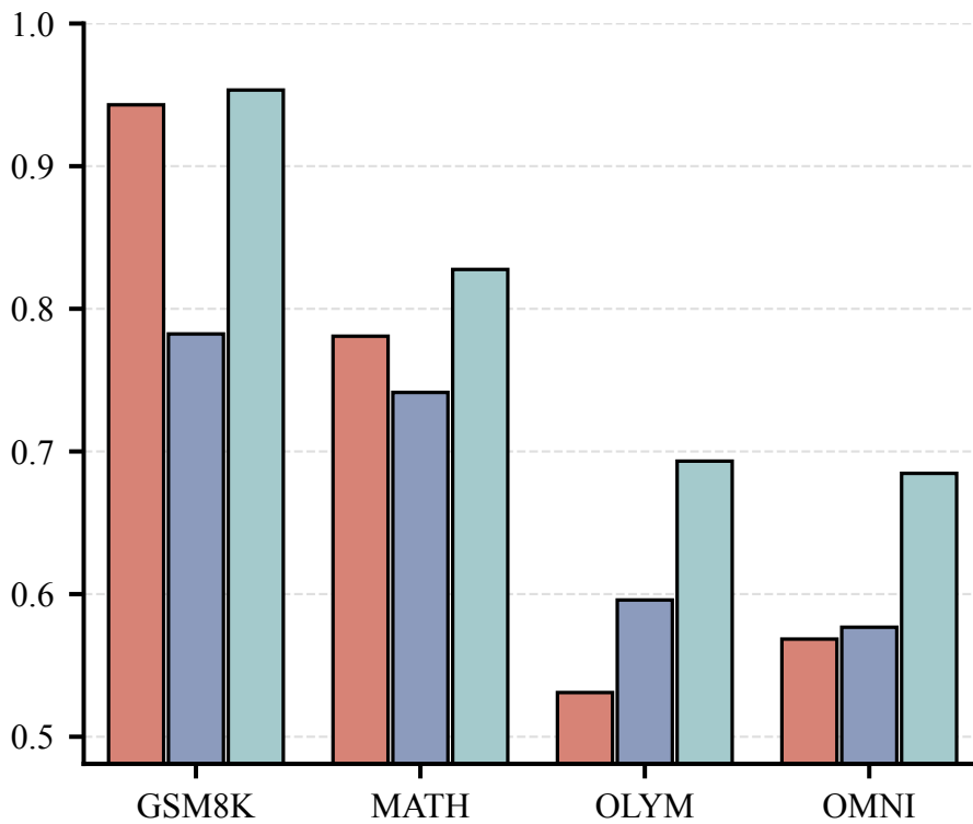
Correct Acc
