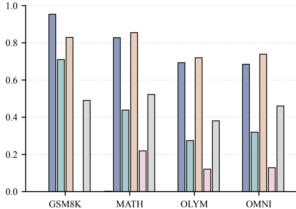
Correct Acc
