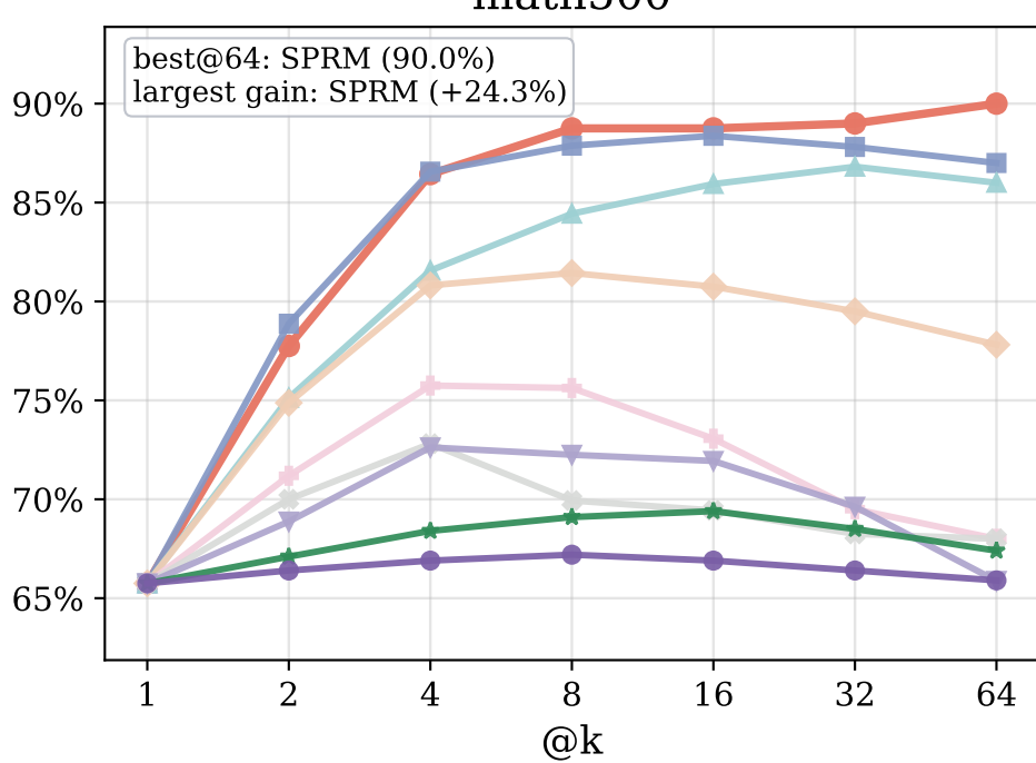
math500
