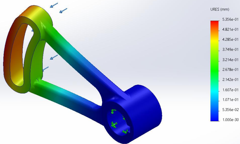
Model_Mania_2008-SimulationXpress Study-Displacement-Displacement
