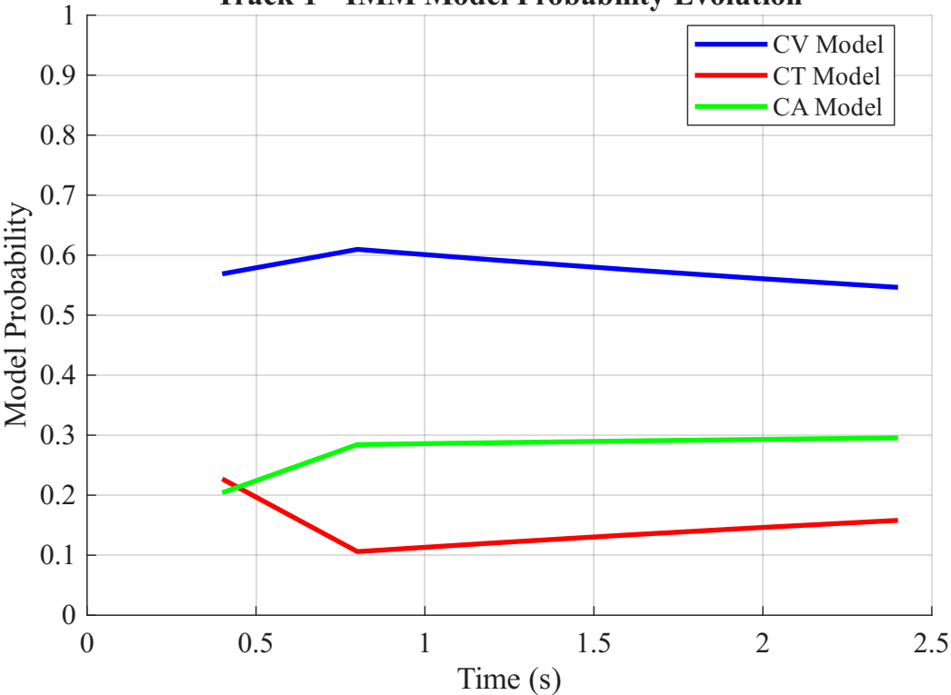
Track 1 - IMM Model Probability Evolution
