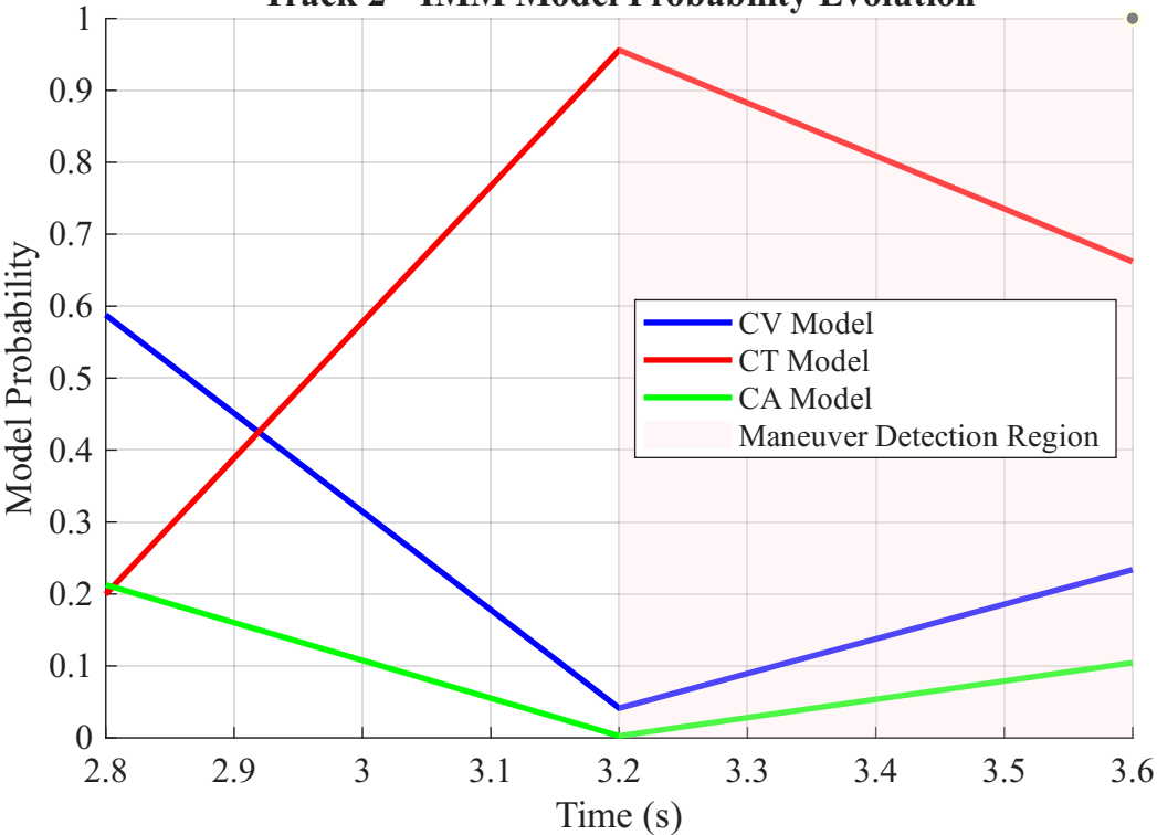
Track 2 - IMM Model Probability Evolution
