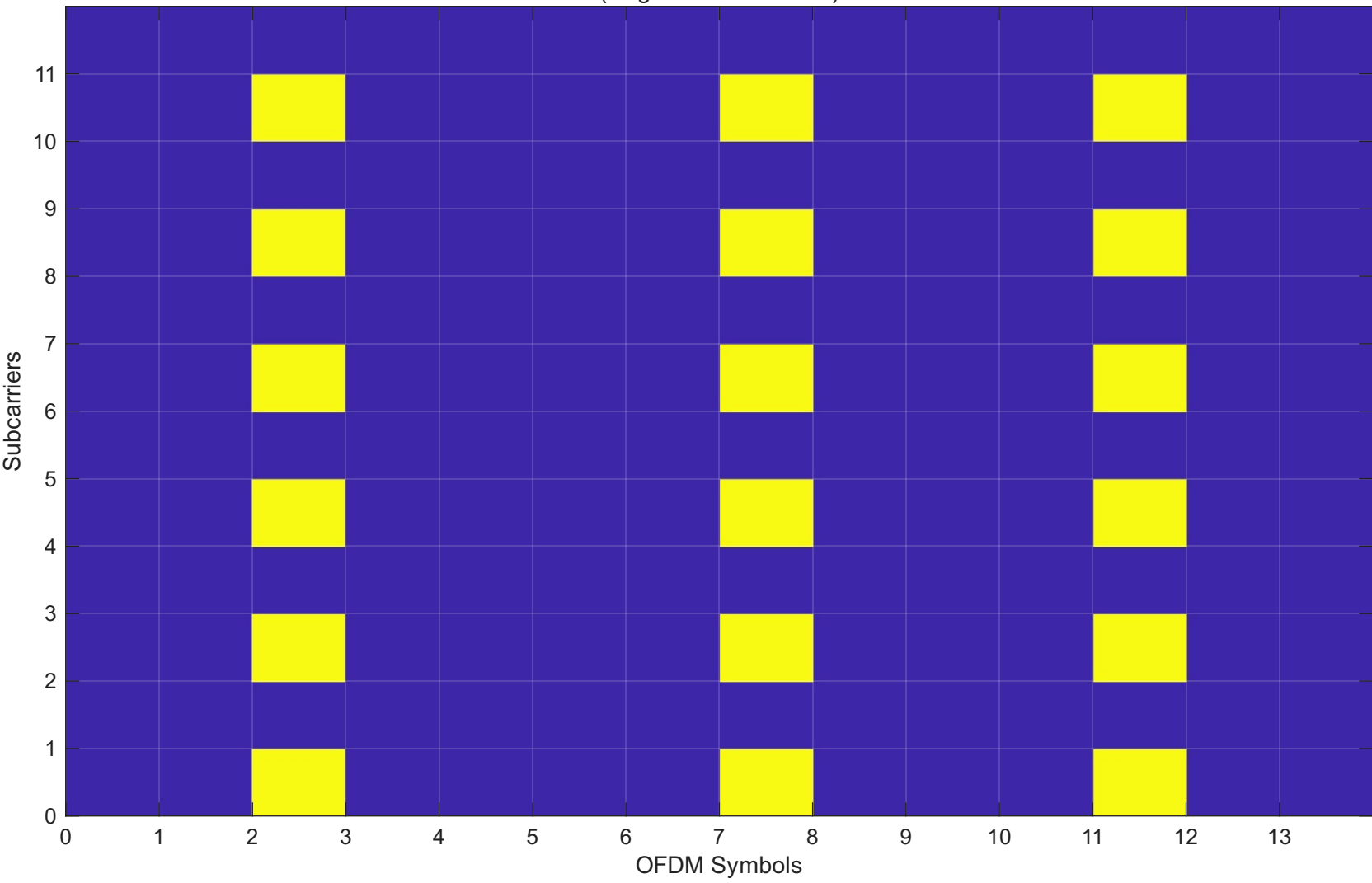
PDSCH DM-RS Resource Elements in the Carrier Resource Grid (single resource block)
